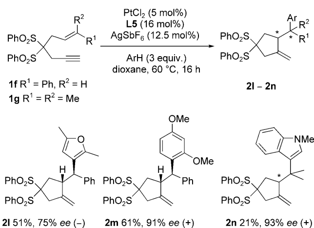
Scheme 3. Platinum-catalyzed asymmetric hydroarylation/cycloisomerization reaction of sulfonated enynes.
