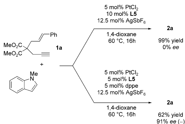
Scheme 4. Pt-catalyzed arylation of enyne 1a .
